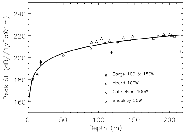
Fig. 6 Observed peak SL-vs-depth of implosion for A19 and near A19-sized bulbs. The solid line represents an approximate fit given by (2).
