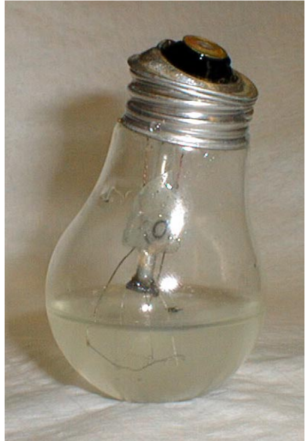
Fig. 1 Photograph of a ceiling fan bulb after pressure testing. Note the water inside the bulb and the crushed base where initial failure occurred. The central filament support 'exploded' under the pressure, but in this case it failed to break the bulb.
