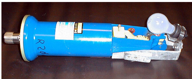
Fig. 9 A mechanical bulb breaker made from a modified acoustic release.
