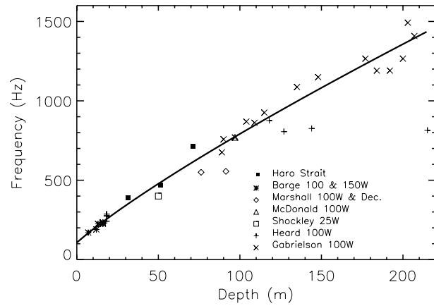
Fig. 5 Observed primary resonant frequency-vs-depth for A19 and near A19-sized bulb. The solid line represents the best fit of (1).
