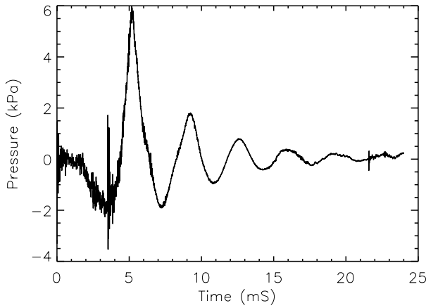
Fig. 2 Time series of a 100W light bulb imploding at a depth of approximately 18.3 m. This waveform was sampled at 256 kHz.
