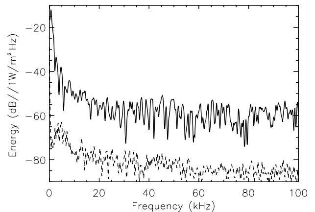
Fig. 3 Solid line represents the energy spectrum of the implosion shown in Fig. 2. Dashed line is the equivalent noise energy at time of measurement.
